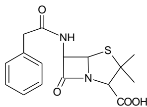
penicillin G
