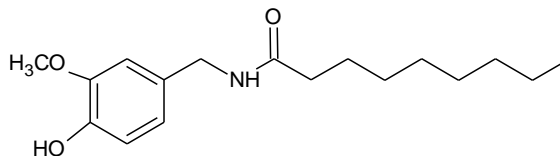
capsaicin
