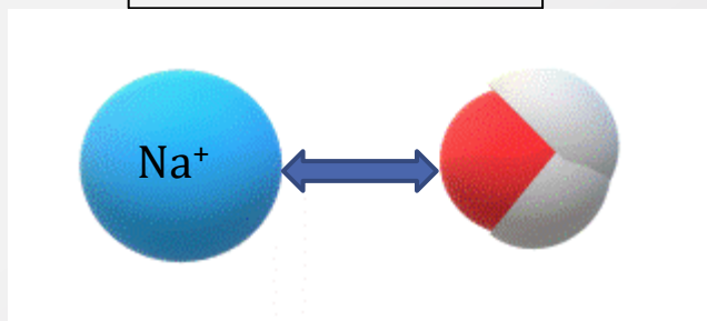
Weak Interaction
