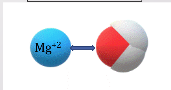
Strong Interaction
